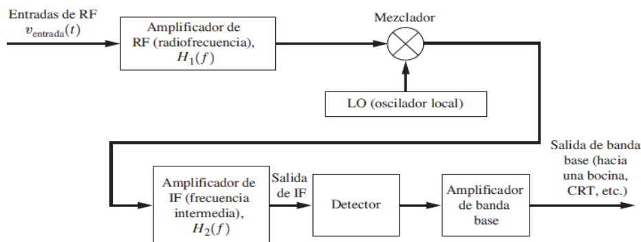
Figura 1. 35: Receptor Superheterodino.
