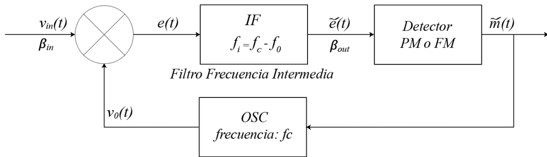
Figura 3.15: Receptor de FMFB.
